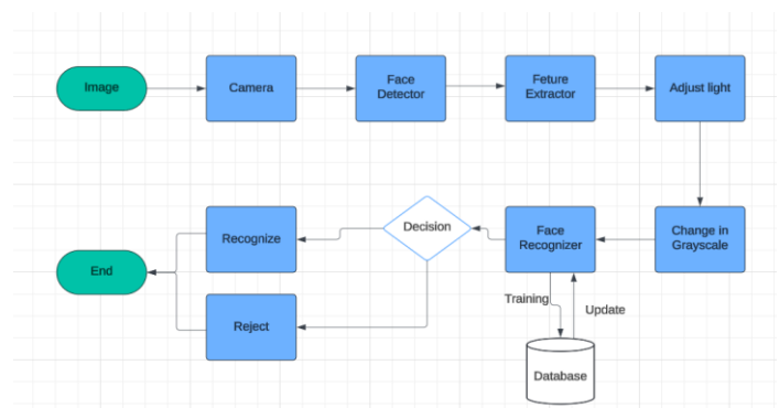
Fig.1 A framework for face recognition system
