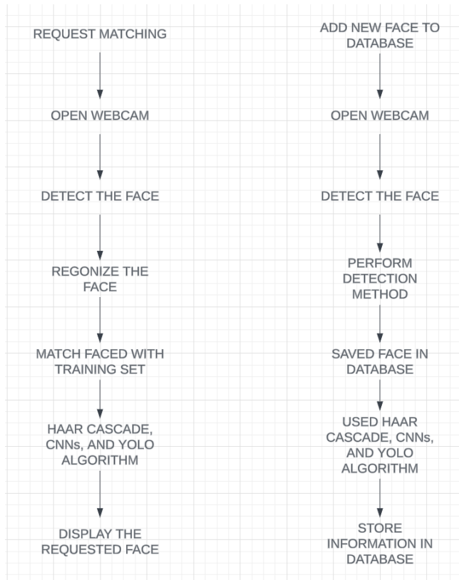
Fig.5 The process of working of algorithm
